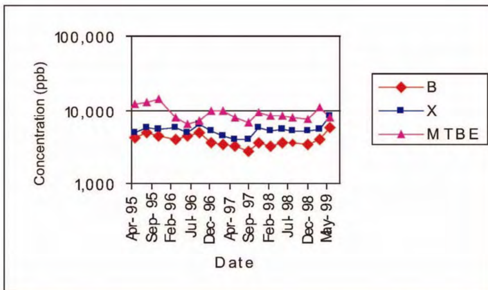
Figure 4-3 Concentrations of MtBE, Benzene, and Xylene in Groundwater in a Monitoring Well with a NAPL Source
