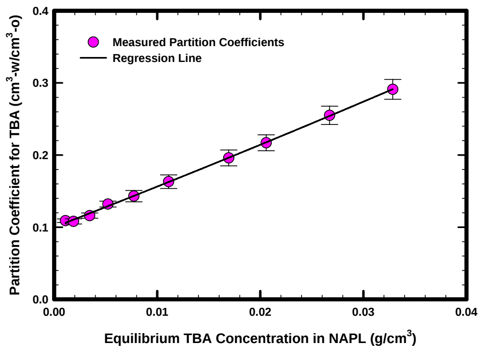
Figure 9a-b. Effect of higher concentrations on partition coefficients for TBA partitioning between a NAPL mixture and an aqueous phase at 24 °C. Partition coefficients are plotted vs. equilibrium aqueous concentration (a) and NAPL concentration (b).
