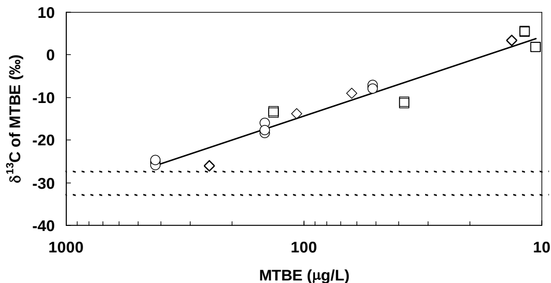
Figure 4-11 Plot of Isotopic Data Demonstrating Natural Biodegradation of MtBE
