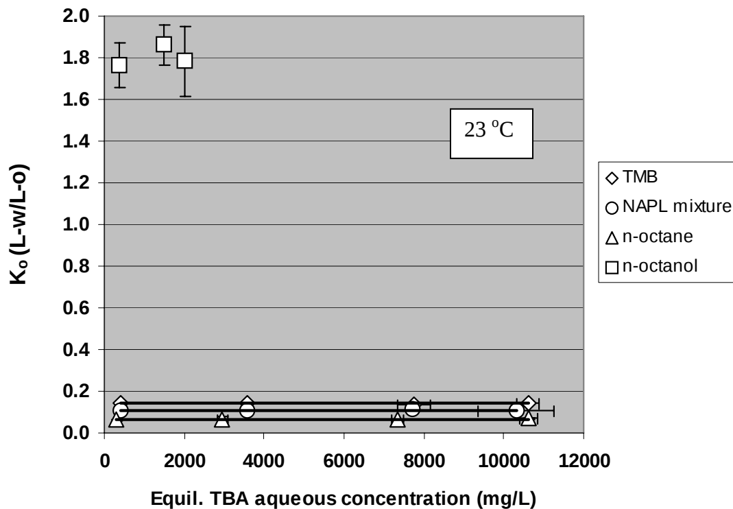
Figure 1. Partition coefficients for TBA partitioning between various NAPLs and an aqueous phase. T=23 °C. Partition coefficients are plotted vs. TBA equilibrium aqueous phase concentrations.
