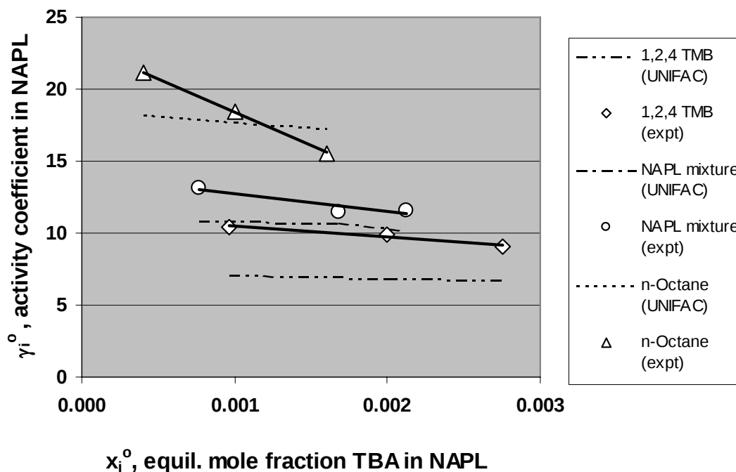
Figure 5. Comparison of UNIFAC calculated and measured activity coefficients for TBA in various NAPLs at 23 °C.
