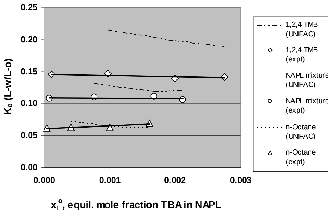
Figure 4. Comparison of UNIFAC calculated and measured partition coefficients for TBA partitioning between various NAPLs and an aqueous phase at 23 °C. Aqueous phase activity coefficients based on literature values (Whitehead and Sandler, 1999); NAPL activity coefficients based on UNIFAC. Aqueous concentration range for UNIFAC calculated curves is limited to the range of literature values for aqueous phase activity coefficients.
