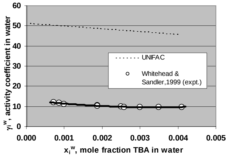
Figure 6. Comparison of UNIFAC calculated and measured activity coefficients for TBA in water at 23 °C.
