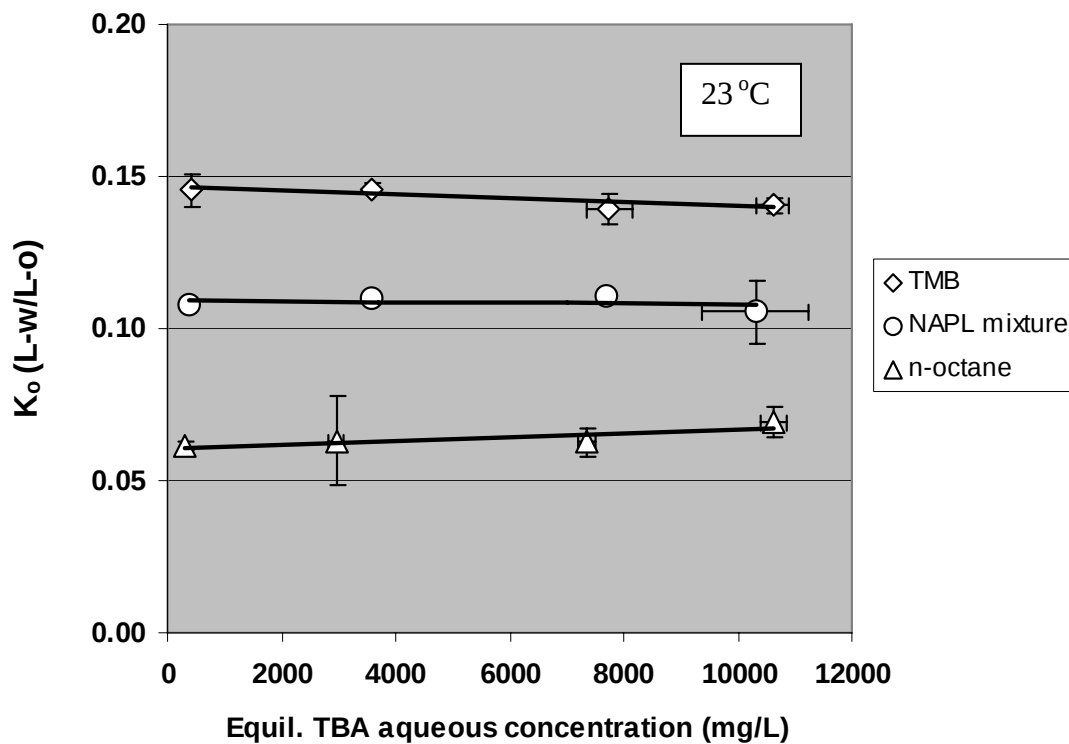
Figure 2. Same as Figure 1 except for expanded scale for TMB, NAPL mixture, and n-Octane.
