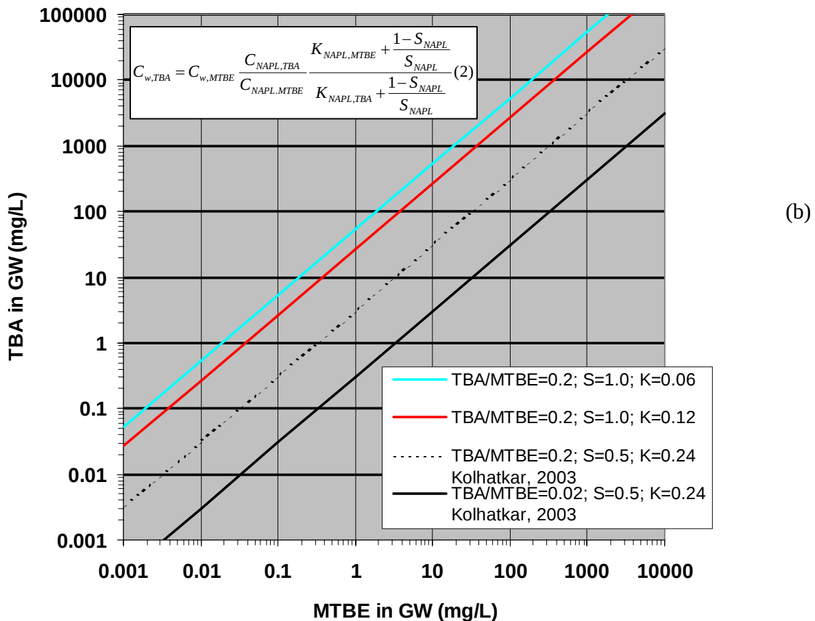
Figures 8a-b. Calculated concentrations of TBA in water vs. MTBE concentrations in ground water near a NAPL source. Calculations are based on Equation 2 for various values of K_{NAPL} for TBA and ratios of concentrations of TBA to MTBE in the NAPL. Figure 8a is reproduced from Kolhatkar, 2003. Curves from 8a are also shown in 8b. Note S_{NAPL}=0.5 corresponds to V_{NAPL}/V_w=1 ; S_{NAPL}=1 corresponds to V_{NAPL}/V_w=\infty .
