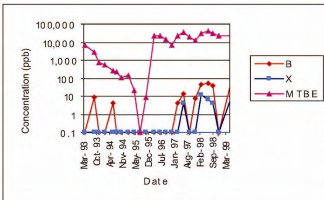
Figure 4-4 Concentrations of MtBE, Benzene, and Xylene in Groundwater in a Monitoring Well with a Vaport Source
